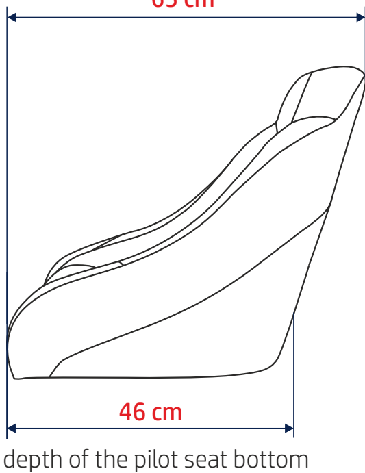
depth of the pilot seat with footrest down 65 cm
