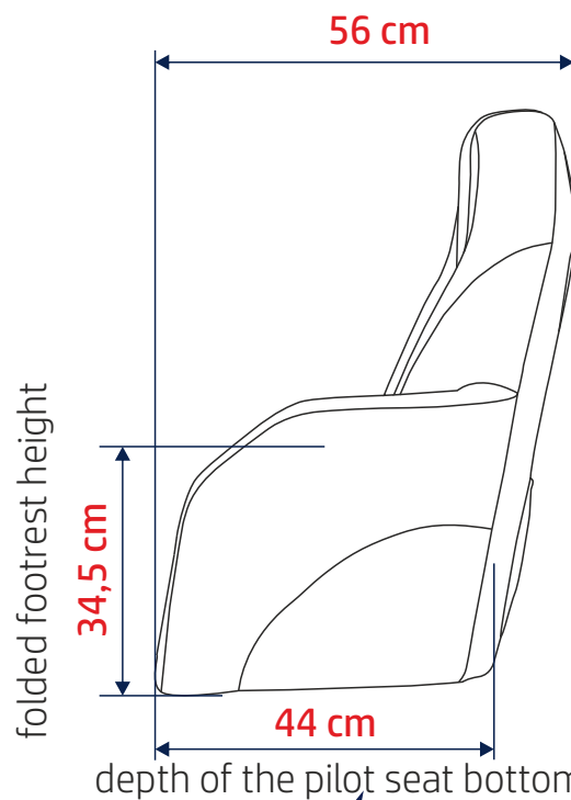
depth of the pilot seat
