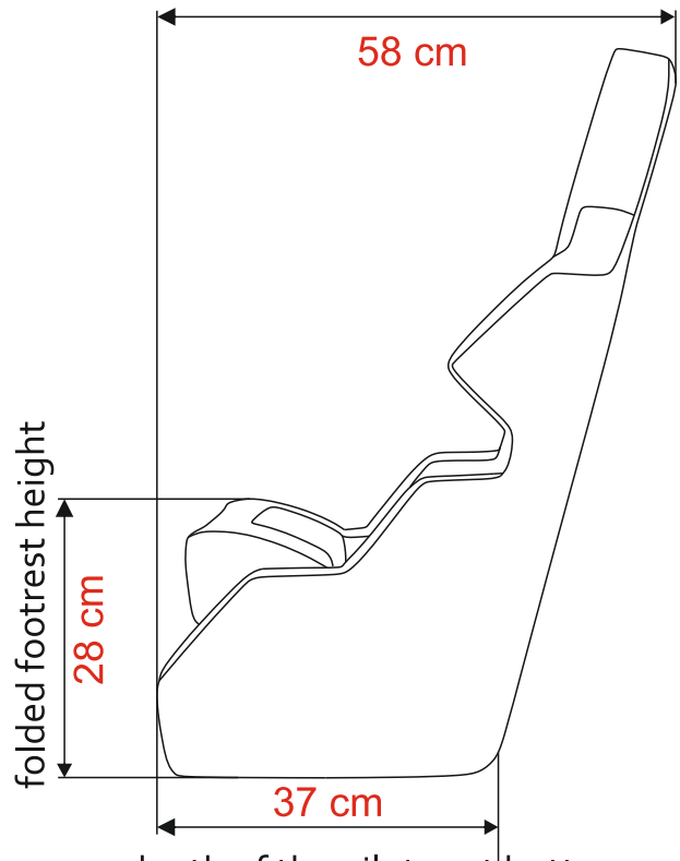
depth of the pilot seat bottom
