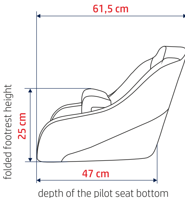
depth of the pilot seat
